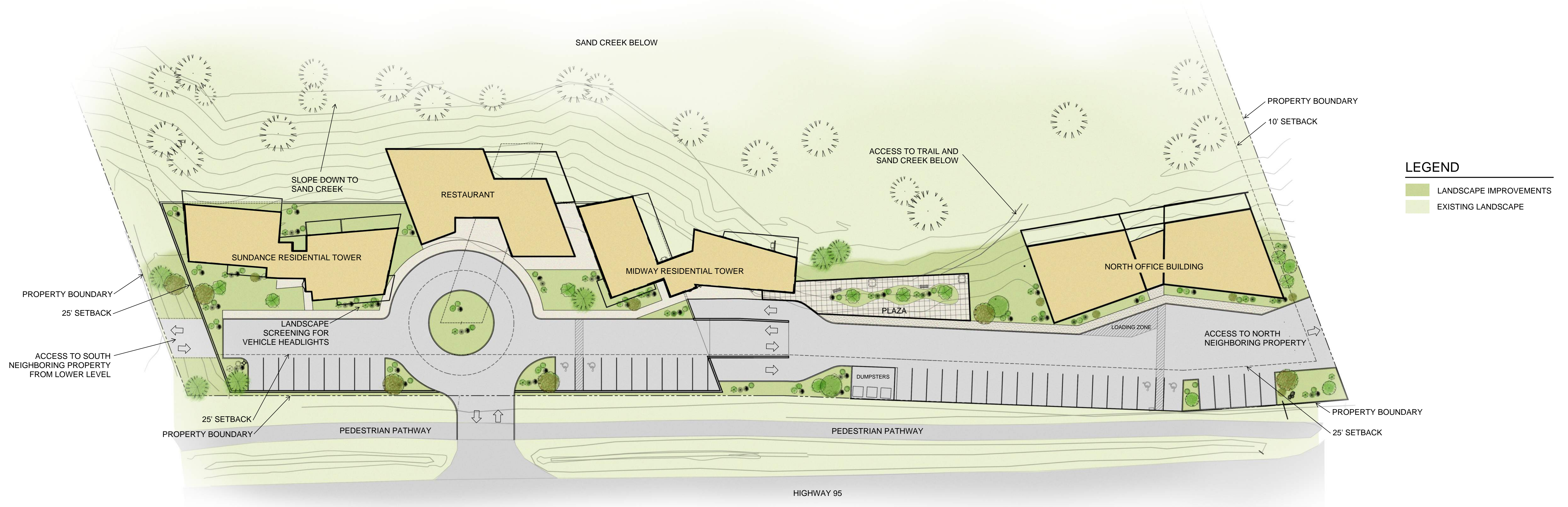
UPPER LEVEL SITE PLAN
