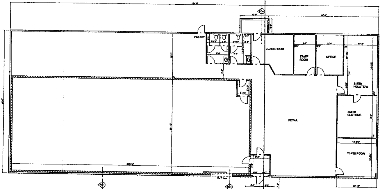
FLOOR PLAN 924417
